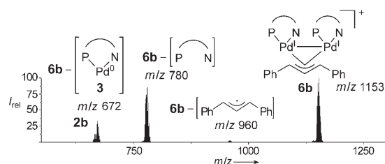
Figure 2. ESI-MS spectrum of dinuclear complex 6b .
